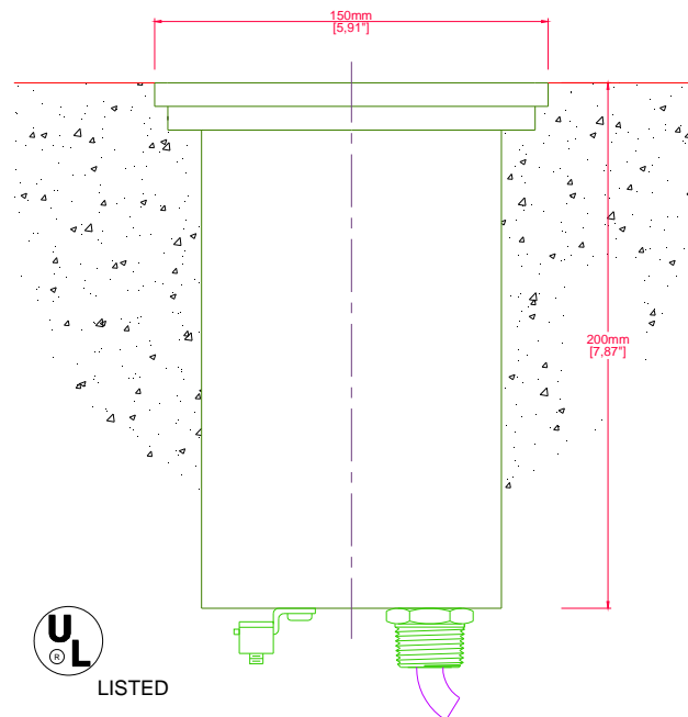
NICHE MOUNTED VERSION SCALE: NONE
