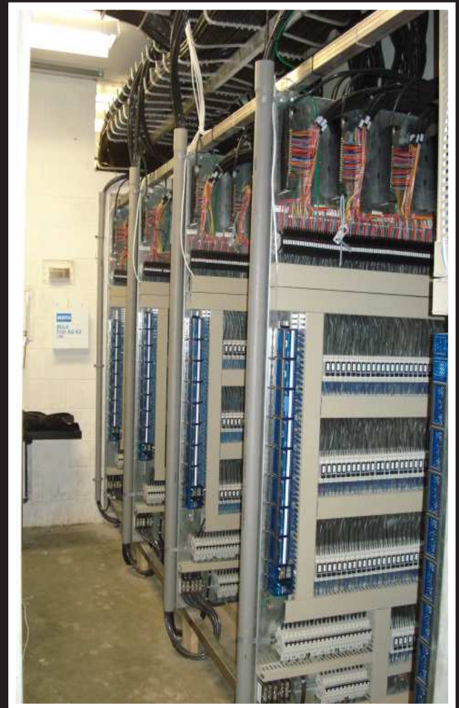
GEFCO Select #EE 950 Show Controller with Sound System
